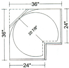
Base Corner BACC3690 Lazy Susan LS3690
